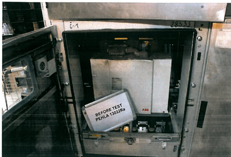
Photo No. 02 Before test PEHLA 13032Ra / 03 Test object, front view with doors of left-hand side panel opened.
